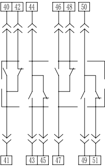
T4-转换4开4闭
