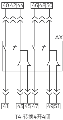
T4-转换4开4闭
