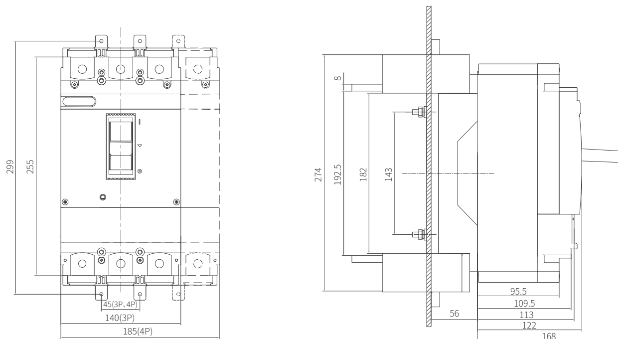
BM5-400/630 插入式外形尺寸图 (3P/4P)
